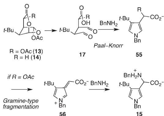
Scheme 9. Mechanistic Outline for Pyrrole Formation from 13 and 14
