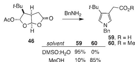
Scheme 11. Conversion of Dioxabicyclo[3.3.0]octanones 46 to Pyrroles 59 and 60
