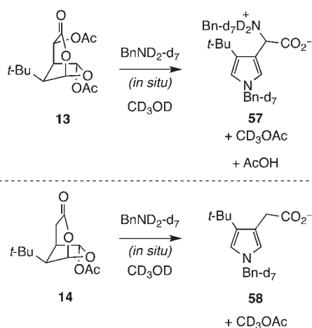
Scheme 10. In Situ Observation of the Formation of 57 and 58 and Reaction Byproducts
