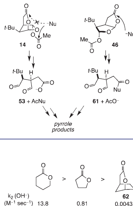
Figure 2. Saponification rates of select lactones. 53
