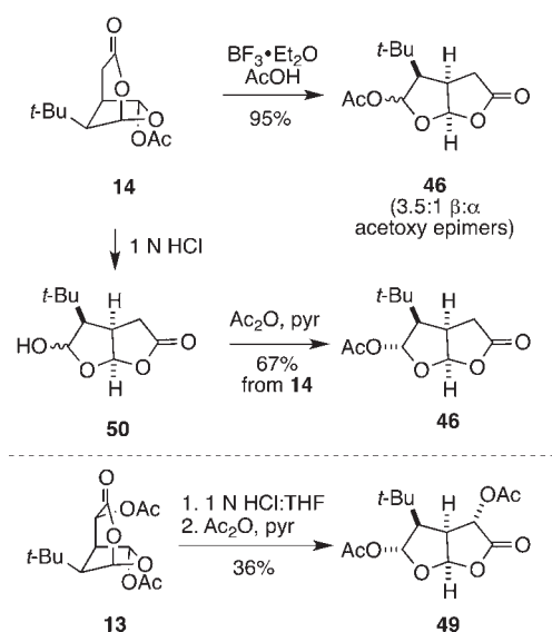
Scheme 7. Conversion of Bridged Dioxabicyclic Lactones 13 and 14 to Fused Isomers 46 and 49
