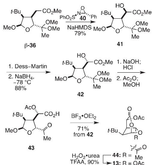
Scheme 5. Completion of the Synthesis of t -Bu-MacE (13)
