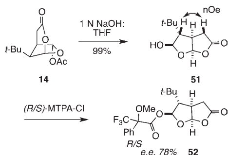
Scheme 8. Synthesis of 51 and Its Mosher Ester
