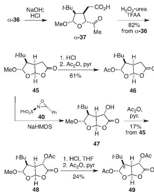
Scheme 6. Synthesis of 2,8-Dioxabicyclo[3.3.0]octanones 46 and 49
